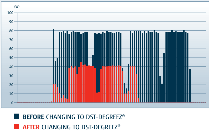
HILDEBRAND A-1476 WASHING PLANT Energy consumption over 24 hours
