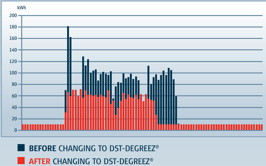
ROLL A-1161 WASHING PLANT Energy consumption over 24 hours
